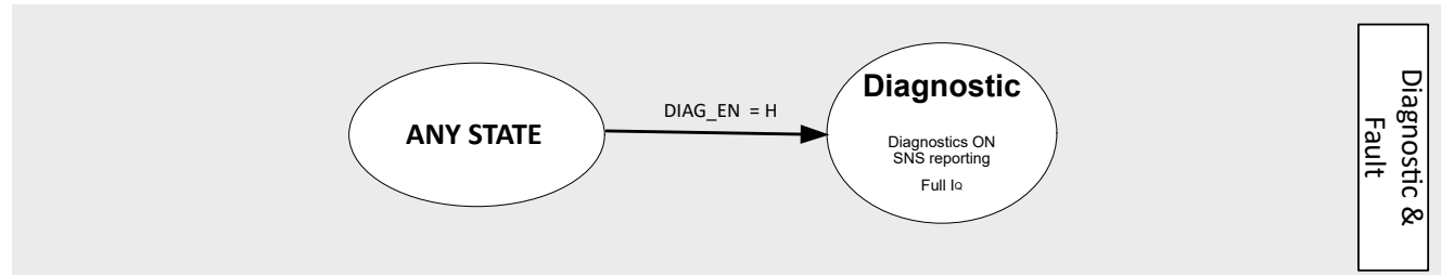
Figure 7-24. State Diagram
