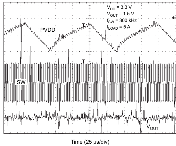
Figure 29. PVDD Hysteresis
