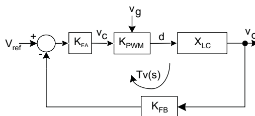
Figure 37. Control Loop
