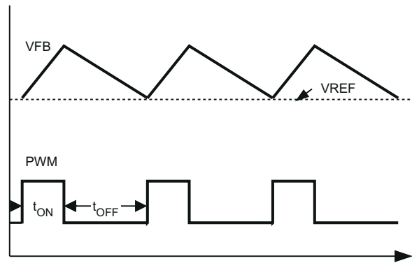
Figure 7-2. On-Time Control Without Ramp Compensation
