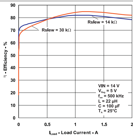
Figure 1. Efficiency vs Load Current for Different Rslew Resistors
