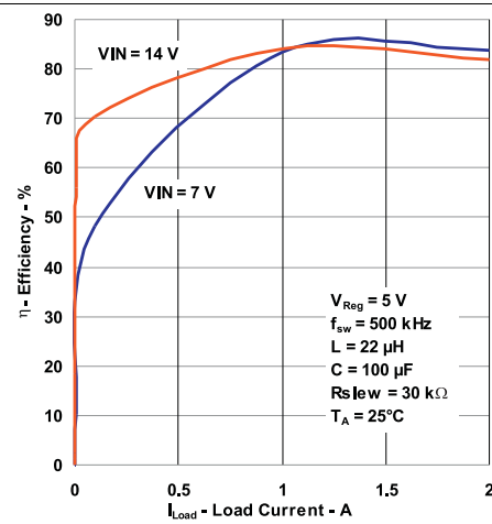
Figure 2. Efficiency vs Load Current for Different Vin
