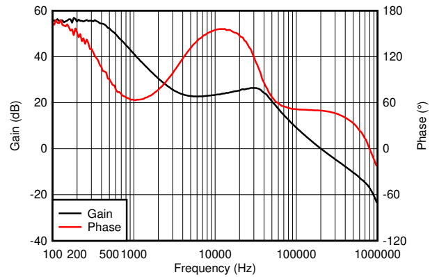
Figure 8-27. Bode Plot
