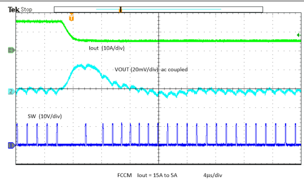
Figure 8-21. Unload Transient
