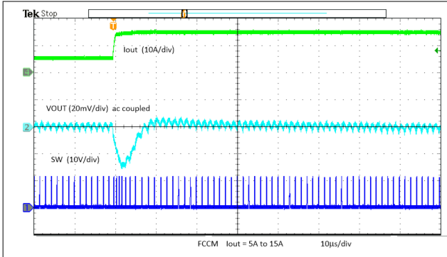
Figure 8-20. Load Transient
