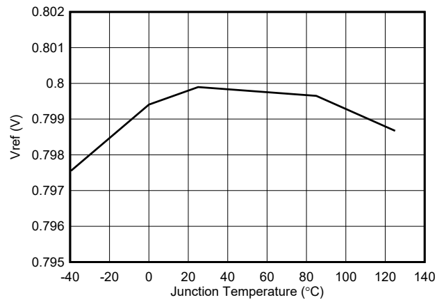
Figure 6-6. V_{REF} Voltage
