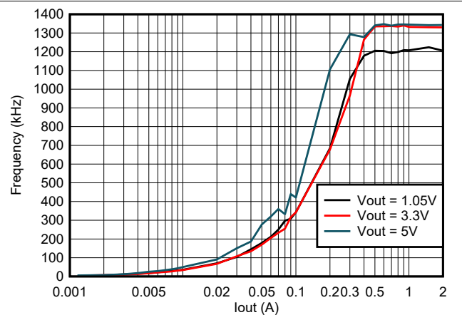
Figure 6-12. Frequency vs Loading, V_{IN} = 12\text{ V}
