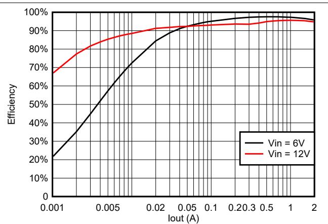
Figure 6-10. Efficiency at 5 V_{OUT} with a 3.3- \mu\text{H} Inductor
