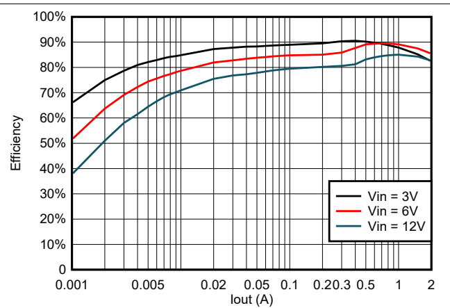
Figure 6-8. Efficiency at 1.05 V_{OUT} with a 1.2- \mu\text{H} Inductor
