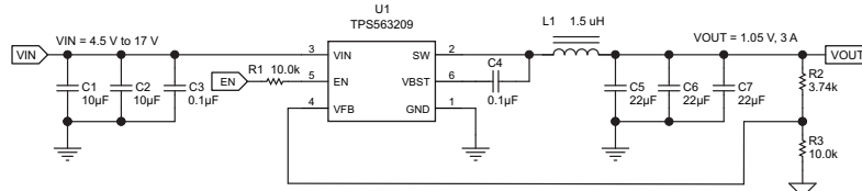
Copyright © 2016, Texas Instruments Incorporated
