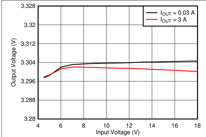
Figure 8-4. Line Regulation
