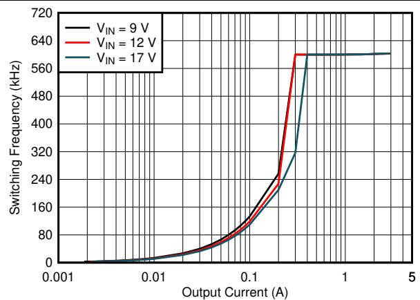
Figure 6-12. Switching Frequency vs Output Current, V_{OUT} = 3.3 \text{ V} , L = 3.3 \mu\text{H}
