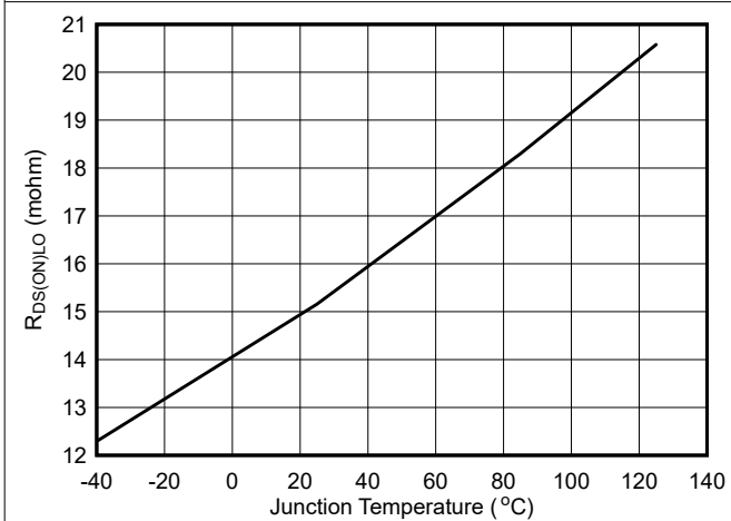
Figure 6-5. Low-Side R_{DS(ON)}
