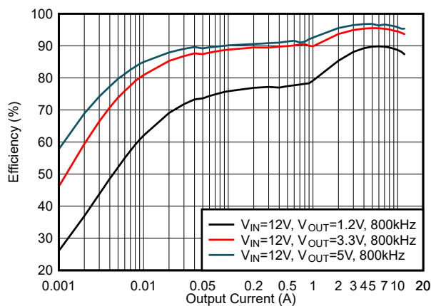
Figure 5-17. Efficiency, DCM Mode, f_{sw} = 800 \text{ kHz}
