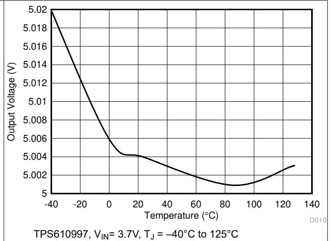
Figure 6-14. Output Voltage vs Temperature
