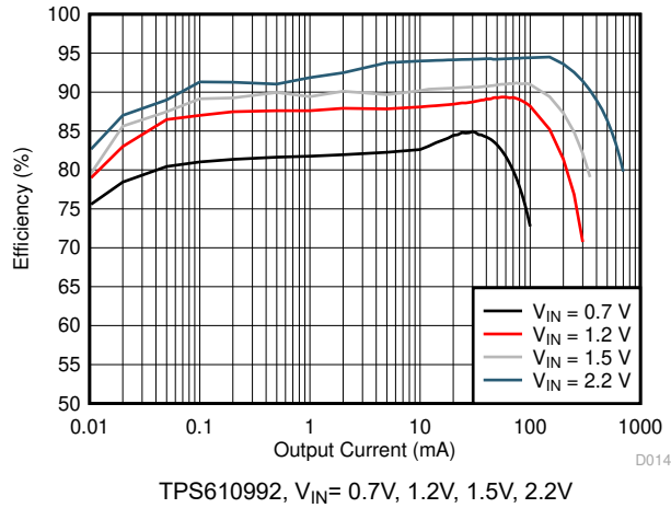
Figure 6-7. TPS610992 Load Efficiency with Different Inputs
