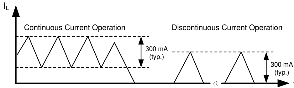
Figure 7-1. Hysteretic Current Operation
