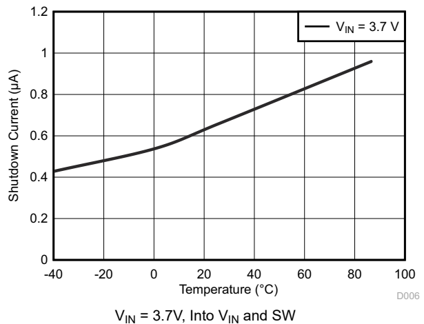
Figure 6-12. Shutdown Current vs Temperature
