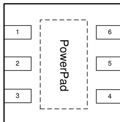
Figure 5-2. DRV Package, 6-Pin WSON (Top View)
