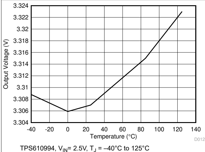
Figure 6-15. TPS610994 Output Voltage vs Temperature
