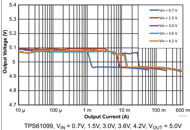
Figure 6-9. Load Regulation
