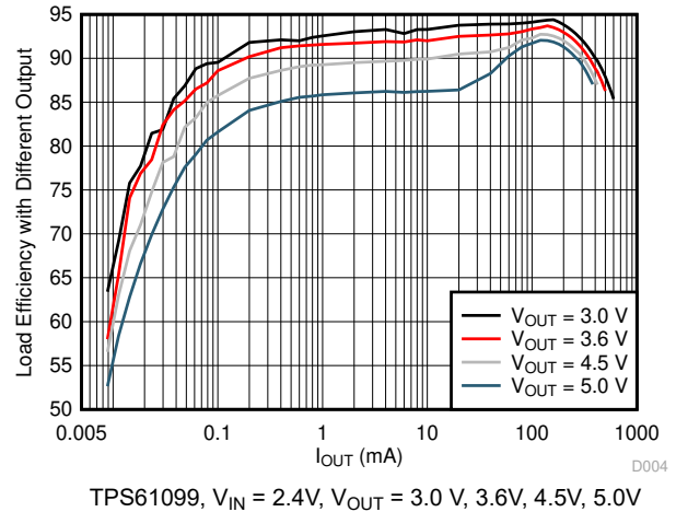
Figure 6-8. Load Efficiency with Different Outputs
