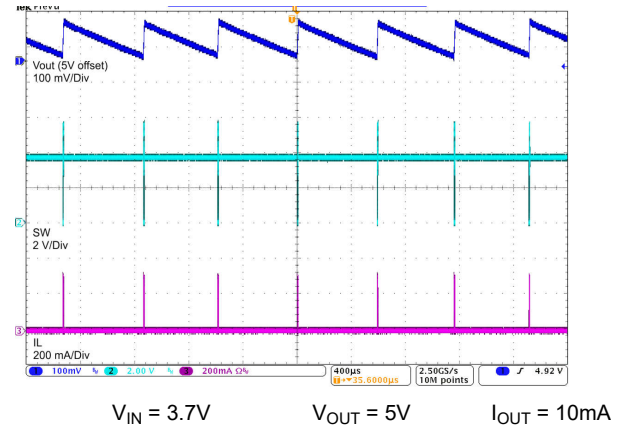
Figure 8-2. Switching Waveform at Light Load
