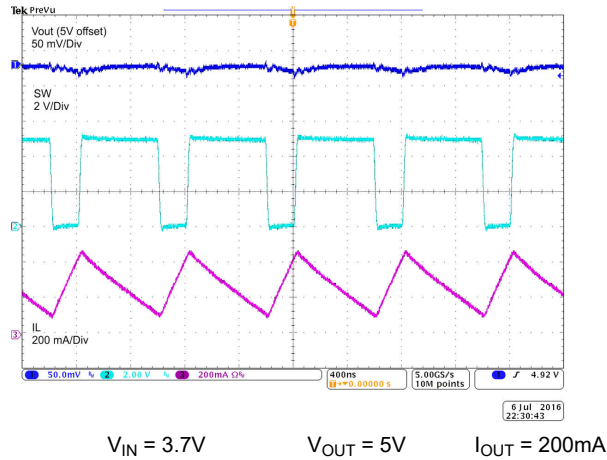
Figure 8-1. Switching Waveform at Heavy Load
