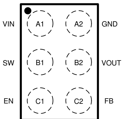
Figure 5-1. YFF Package, 6-Pin DSBGA (Top View)
