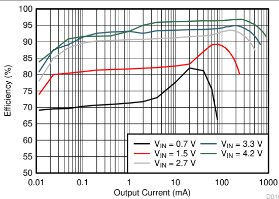
TPS610996, V_{IN} = 0.7V, 1.5V, 2.7, 3.3V, 4.2V
