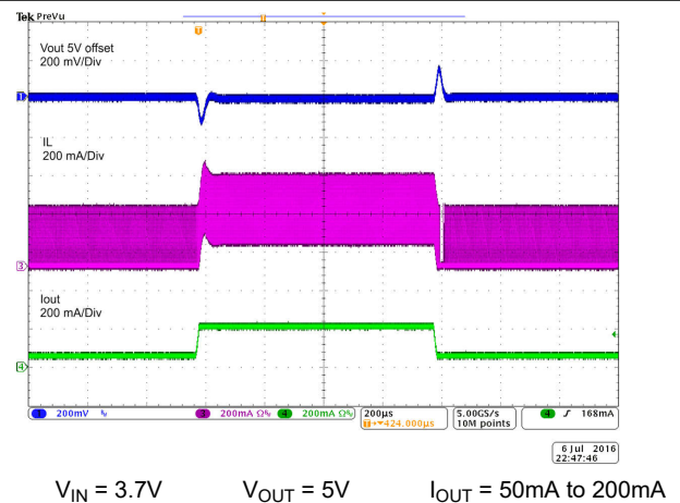
Figure 8-6. Load Transient
