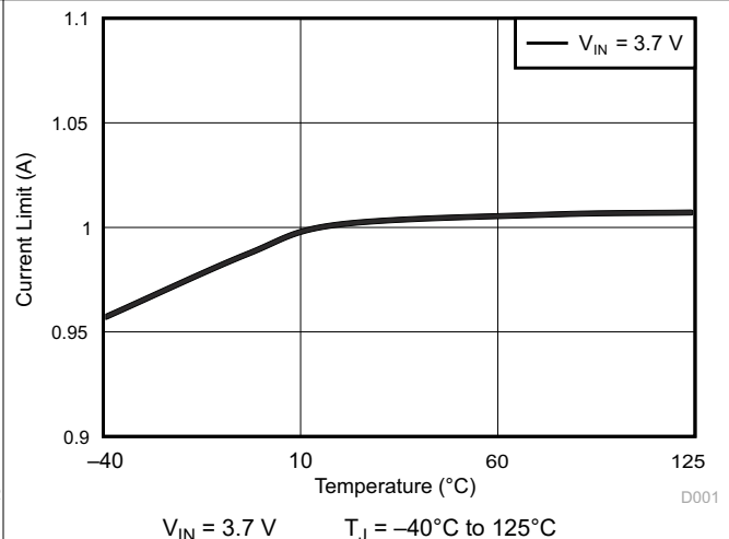
Figure 6-16. Current Limit vs Temperature
