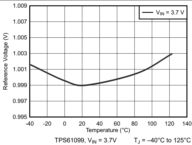
Figure 6-13. Reference Voltage vs Temperature
