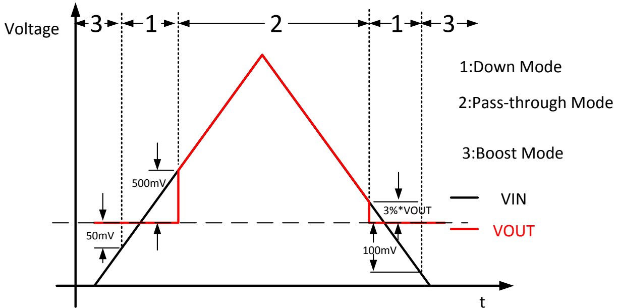
Figure 7-3. Down Mode and Pass-Through Operation
