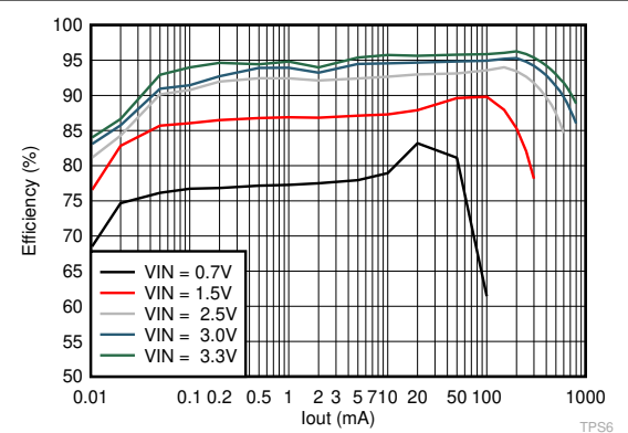
TPS610995, V_{IN} = 0.7V, 1.5V, 2.0, 3.0V, 3.3V
