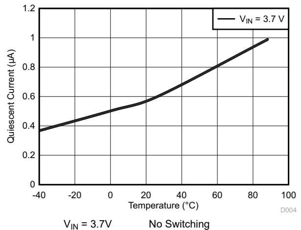
Figure 6-10. Quiescent Current into V_{OUT} vs Temperature
