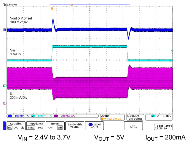
Figure 8-5. Line Transient
