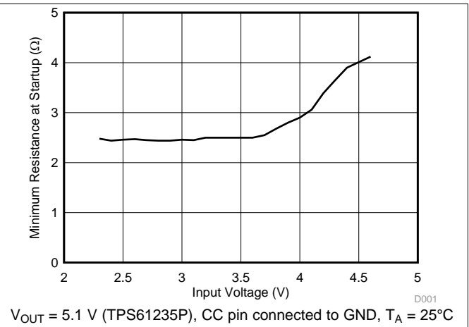
Figure 8. Minimum Load Resistance at Startup
