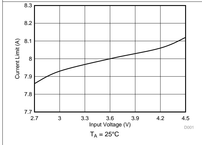
Figure 9. Current Limit vs Input Voltage
