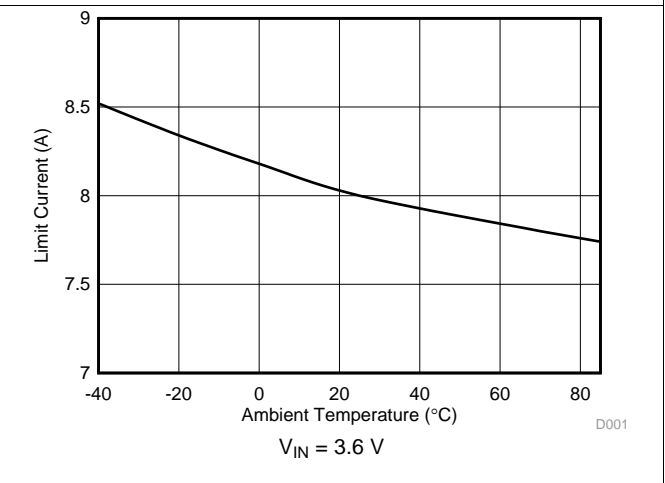
Figure 10. Current Limit vs Ambient Temperature
