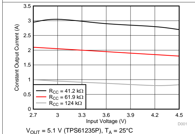
Figure 11. Constant Output Current vs Input Voltage
