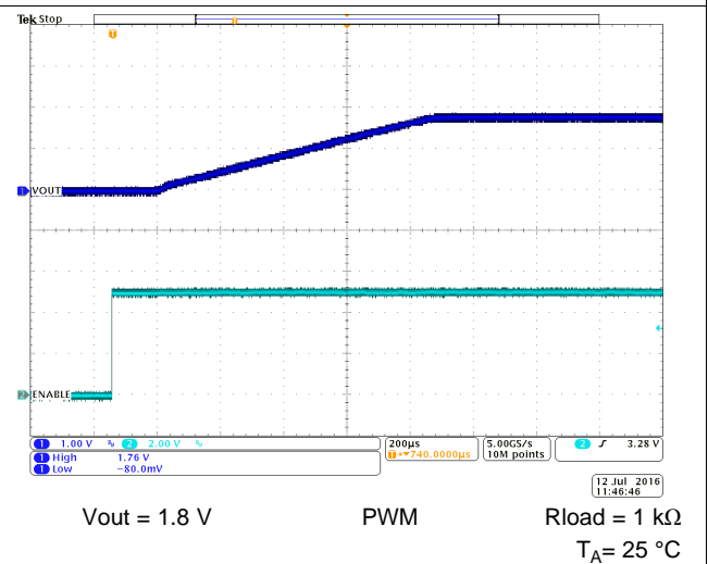
Figure 47. Start-Up Timing
