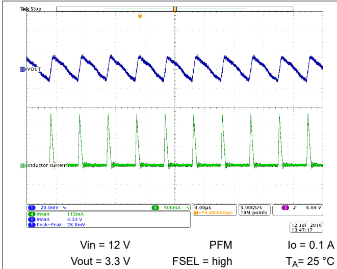
Figure 10-50. Output Voltage Ripple
