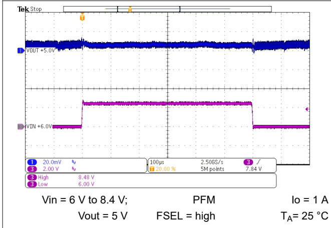
Figure 10-54. Line Transient Response
