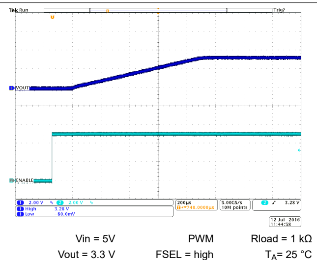
Figure 10-49. Start-Up Timing
