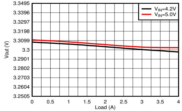
Figure 8-22. Load Regulation
