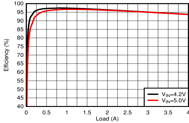
Figure 8-21. PWM Efficiency
