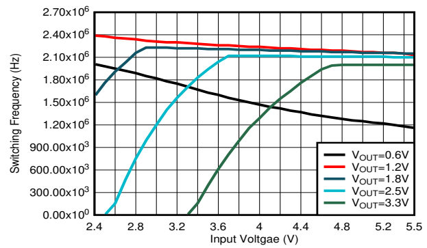
Figure 8-26. Switching Frequency
