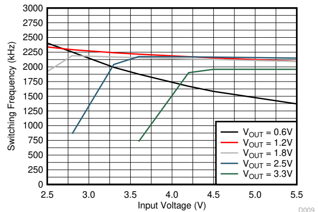
Figure 8-24. Switching Frequency
