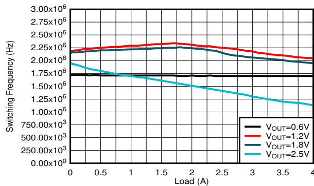
Figure 8-25. Switching Frequency
