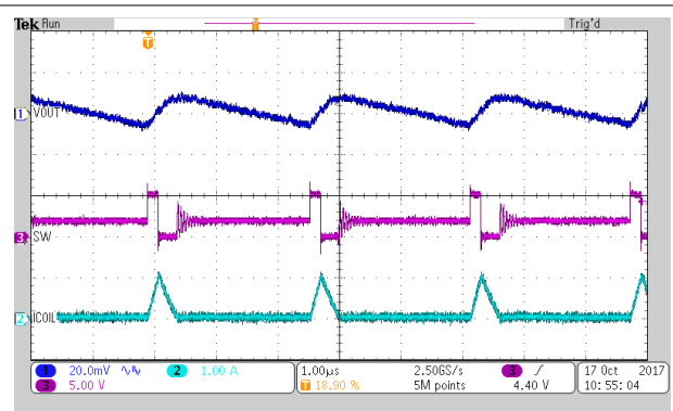
I_{OUT} = 0.1A TPS62824/5/6/7 Figure 8-34. PSM Operation
