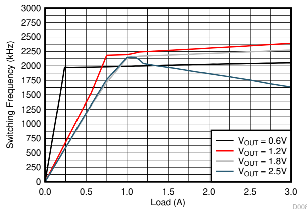
Figure 8-23. Switching Frequency
