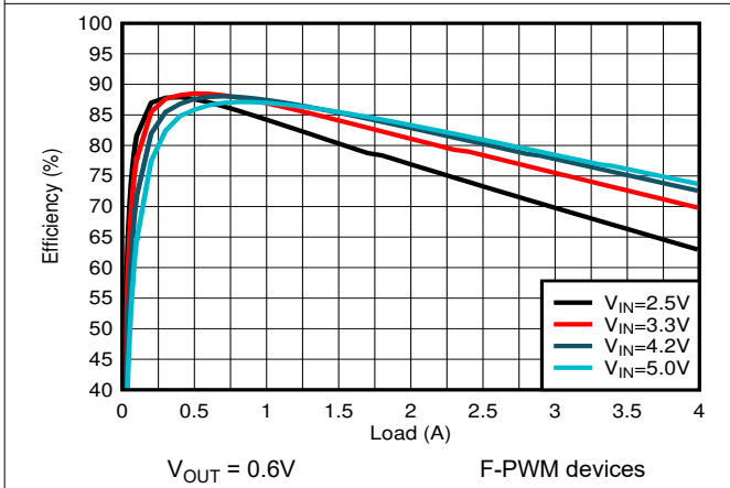
Figure 8-5. PWM Efficiency
