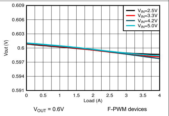
Figure 8-6. Load Regulation
