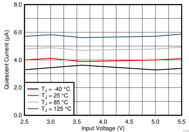
Figure 6-4. Quiescent Current
