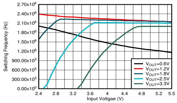
I_{OUT} = 1.0A TPS62824A/5A/6A/7A Figure 8-26. Switching Frequency
