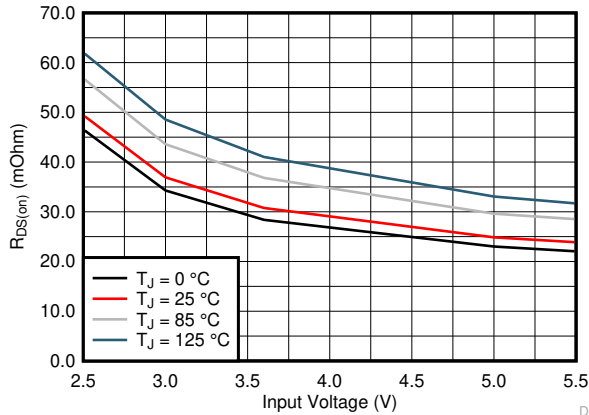
Figure 6-1. High-Side FET On-Resistance
