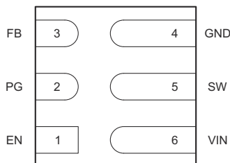
Figure 5-1. DMQ Package, 6-Pin VSON-HR (Bottom View)
