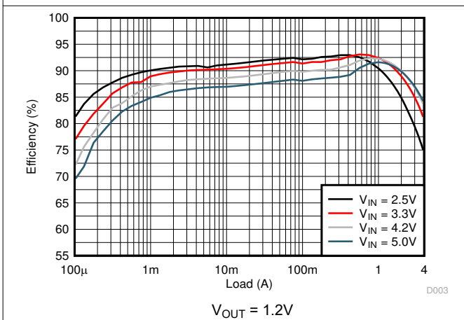
Figure 8-7. Efficiency
