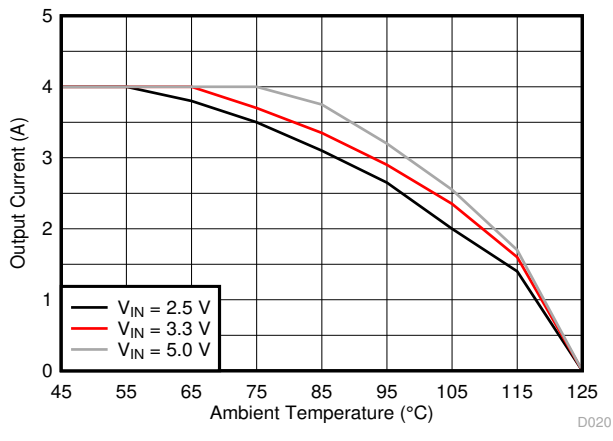
Figure 8-29. Thermal Derating
