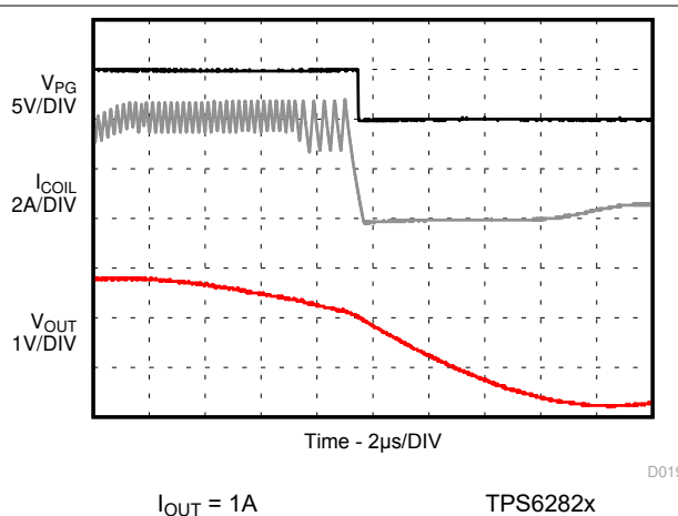
Figure 8-48. HICCUP Short-Circuit Protection (Zoom In)
