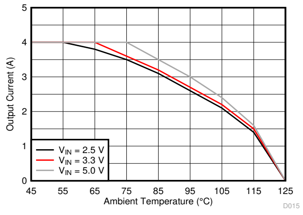
Figure 8-30. Thermal Derating
