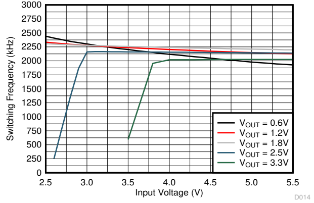
Figure 8-28. Switching Frequency
