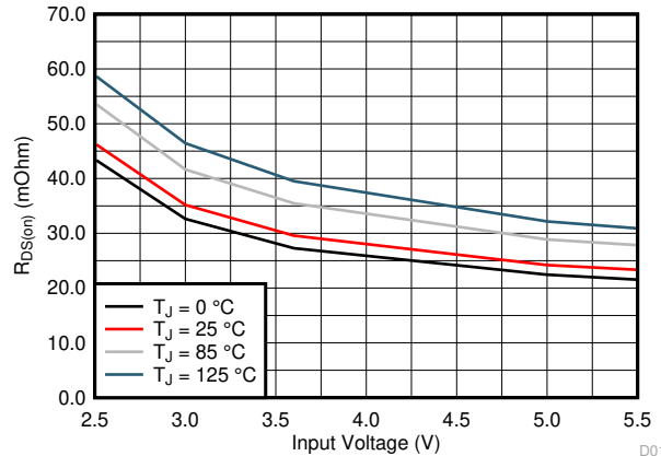
Figure 6-2. Low-Side FET On-Resistance
