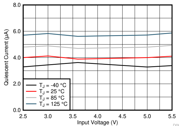
Figure 6-4. Quiescent Current
