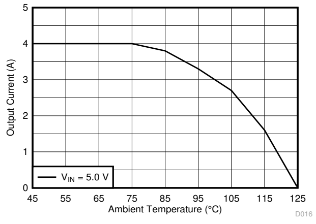
Figure 8-32. Thermal Derating
