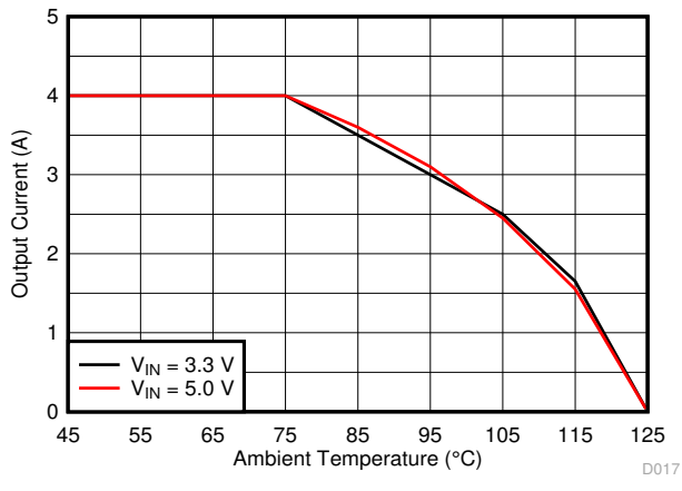
Figure 8-31. Thermal Derating
