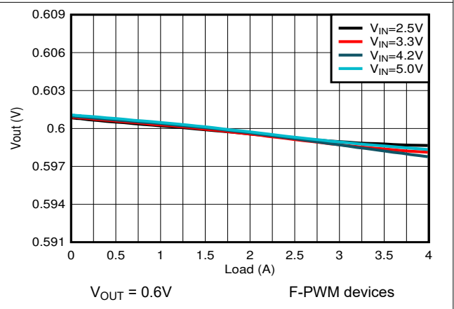
Figure 8-6. Load Regulation
