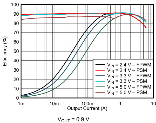
Figure 9-4. Efficiency
