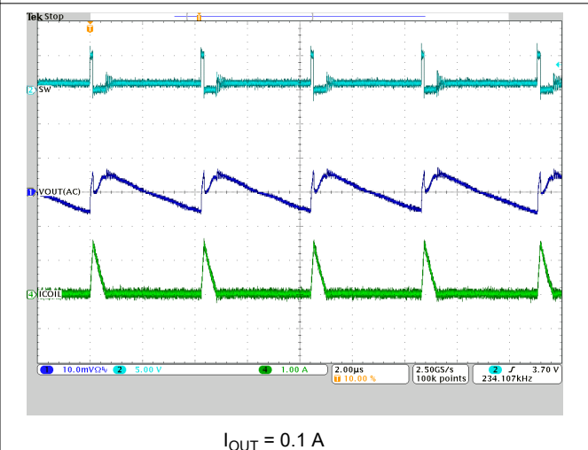
Figure 9-15. Switching Frequency
