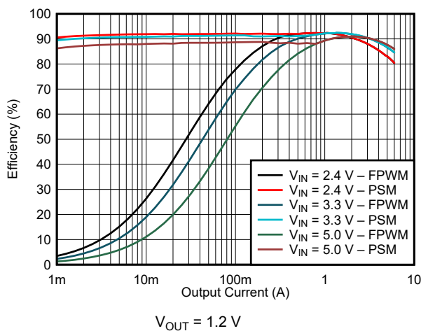
Figure 9-6. Efficiency
