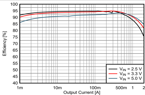
Figure 8-16. 0.6V Output Efficiency
