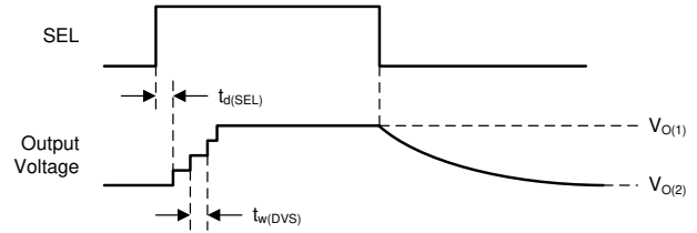
Figure 6-11. Dynamic Voltage Scaling with Light Load
