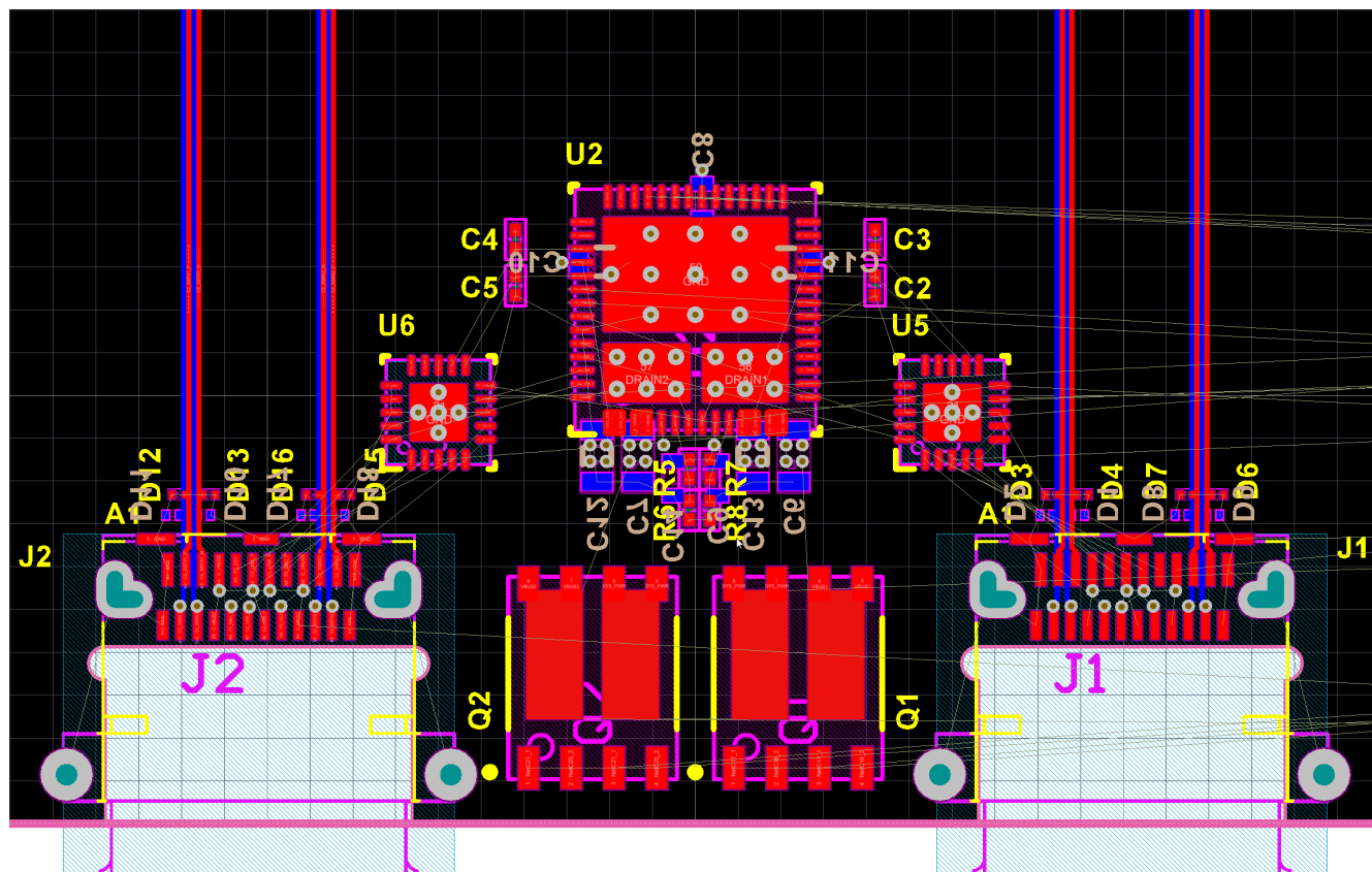
Figure 11-13. Protection Placement
