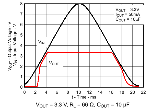
Figure 6-18. Power-Up and Power-Down for New Chip
