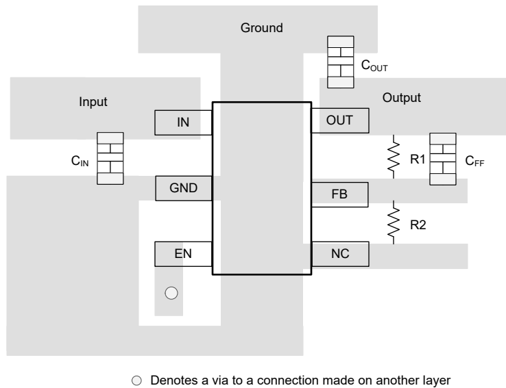
Figure 7-9. Layout Example (DBV Adjustable Package, New Chip)
