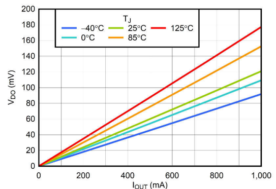
Figure 5-6. Dropout Voltage vs Output Current New silicon, M3 suffix
