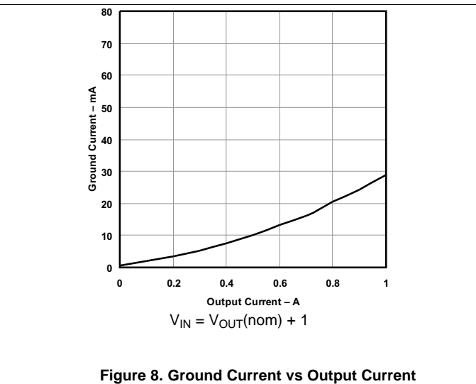
Figure 8. Ground Current vs Output Current
