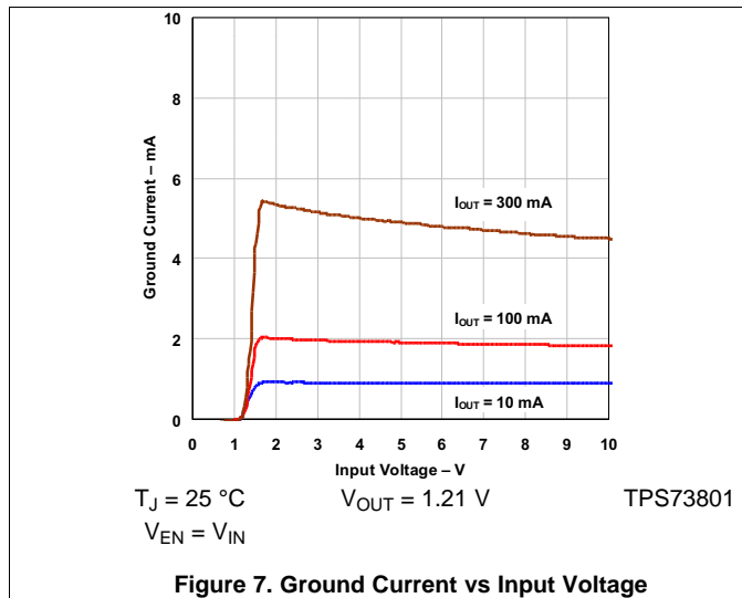
Figure 7. Ground Current vs Input Voltage
