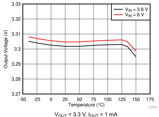
Figure 6-2. Output Voltage vs Ambient Temperature
