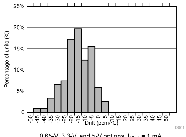
Figure 6-4. Temperature Drift Histogram ( -40^\circ\text{C} to +25^\circ\text{C} )
