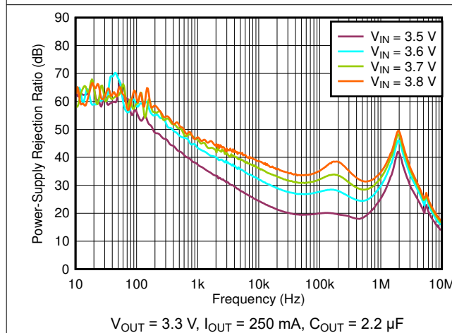
Figure 5-33. PSRR vs Frequency and V_{IN}
