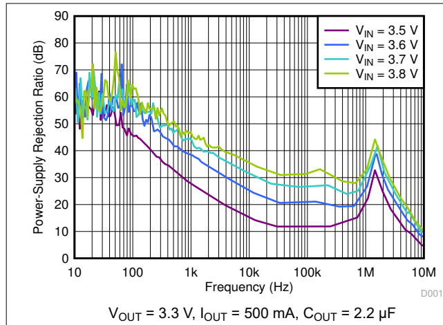
Figure 5-31. PSRR vs Frequency and V_{IN}
