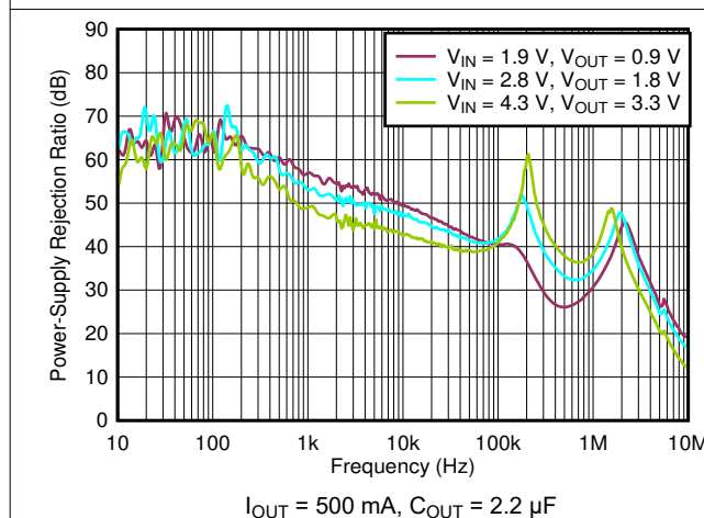
Figure 5-35. PSRR vs Frequency
