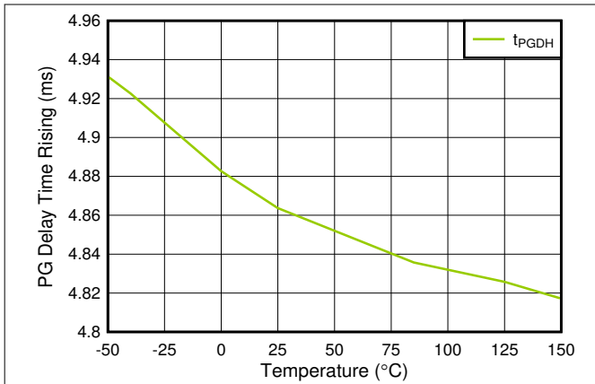
Figure 5-19. t_{PGDH} vs Temperature (For TPS746B Only)
