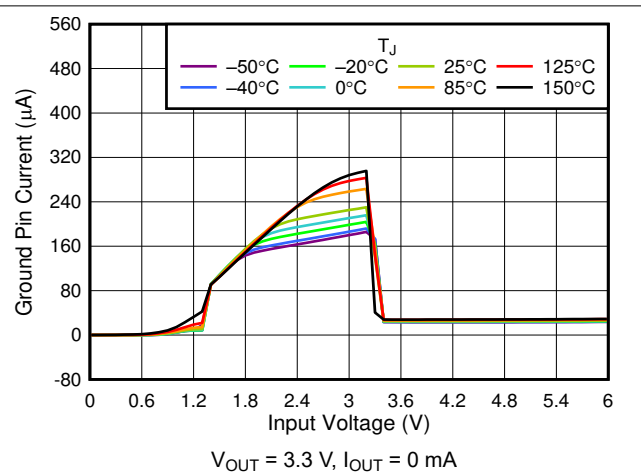
Figure 5-10. I_{GND} vs V_{IN}
