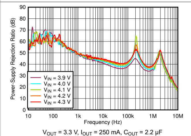
Figure 5-34. PSRR vs Frequency and V_{IN}
