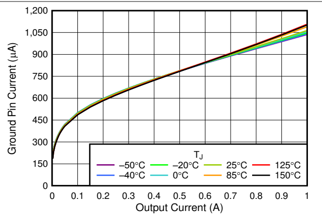
Figure 5-8. I_{GND} vs I_{OUT}
