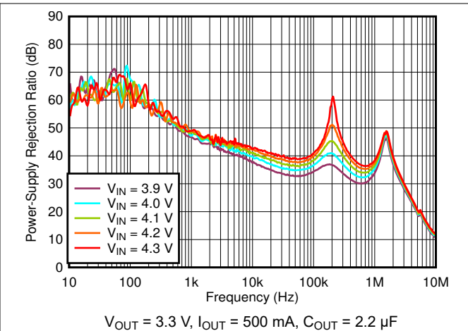
Figure 5-32. PSRR vs Frequency and V_{IN}
