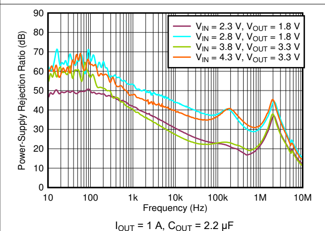
Figure 5-36. PSRR vs Frequency
