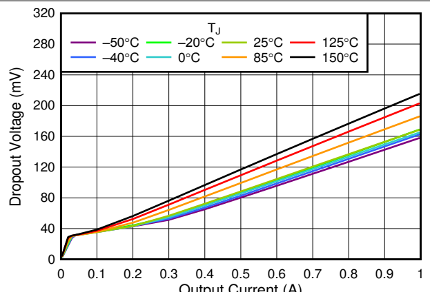
Figure 6-4. 3.3-V Dropout Voltage vs I_{OUT}
