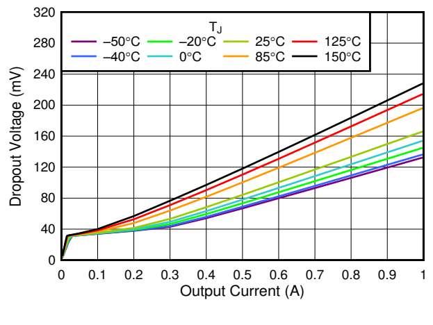
Figure 6-4. 3.3-V Dropout Voltage vs I_{OUT}
