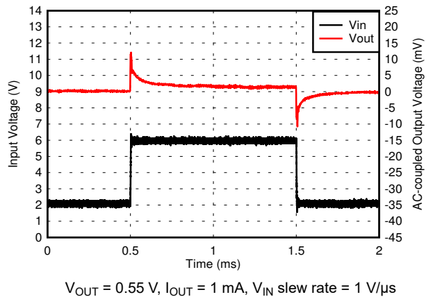
Figure 6-24. 0.55-V Line Transient
