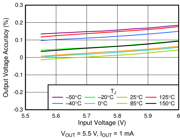
Figure 6-3. 5.5-V Line Regulation vs V_{IN}
