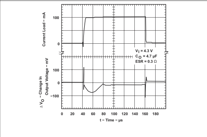
Figure 5-42. TPS76933 Load Transient Response (Legacy Chip)
