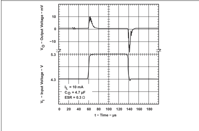
Figure 5-39. TPS76933 Line Transient Response (Legacy Chip)
