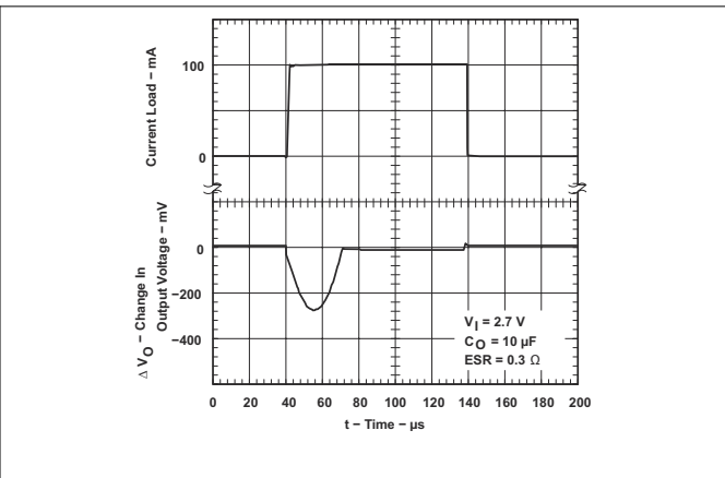
Figure 5-38. TPS76915 Load Transient Response (Legacy Chip)
