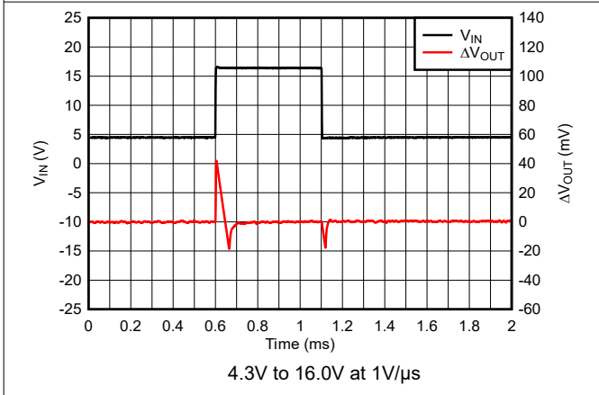
Figure 5-41. TPS76933 Line Transient Response (New Chip)
