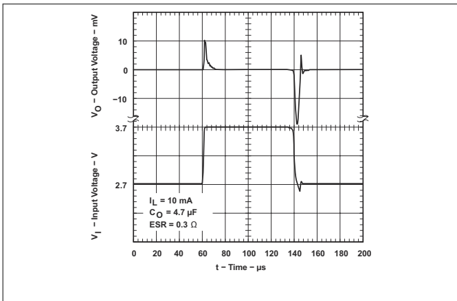
Figure 5-37. TPS76915 Line Transient Response (Legacy Chip)
