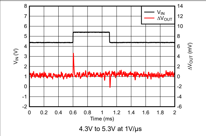
Figure 5-40. TPS76933 Line Transient Response (New Chip)
