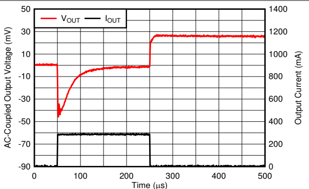
Figure 6-58. Load Transient
