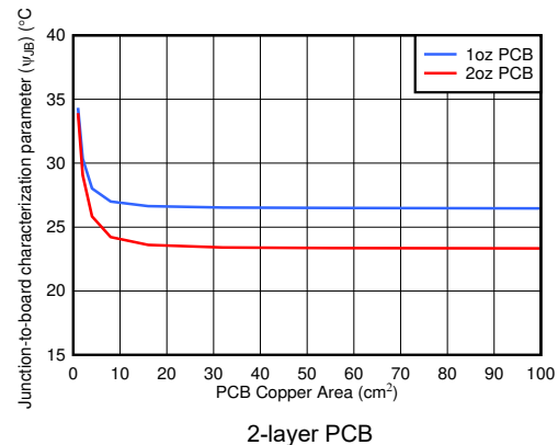
Figure 10-4. Junction-to-Board Characterization Parameter ( \psi_{JB} ) vs PCB Copper Area
