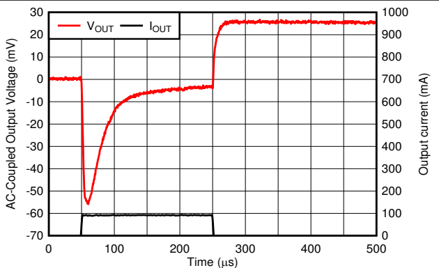
Figure 6-56. Load Transient
