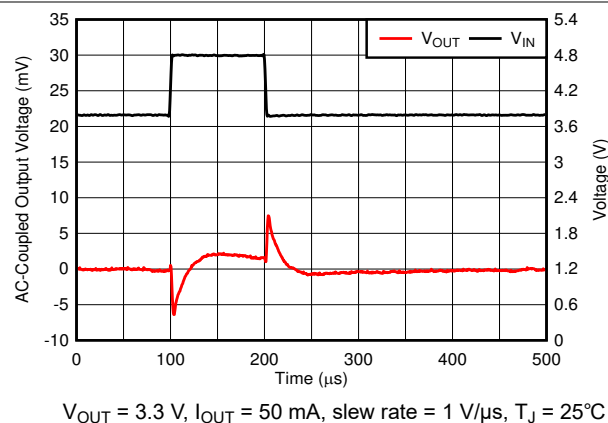
Figure 6-35. Line Transient
