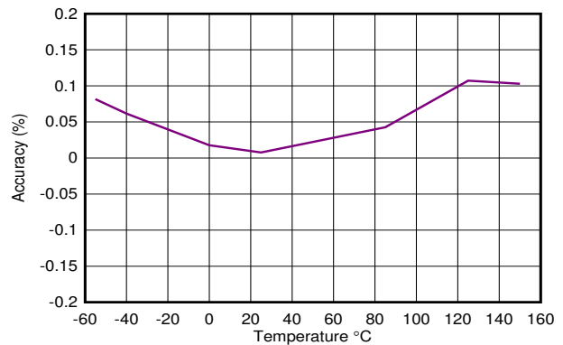
Figure 6-8. Accuracy vs Temperature
