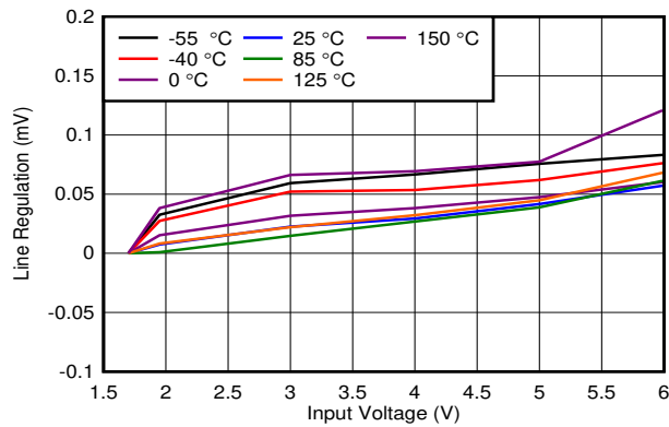
Figure 6-7. 50-mA Line Regulation
