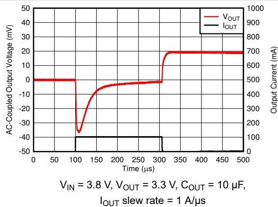
Figure 8-9. I_{OUT} Transient From 0 mA to 100 mA
