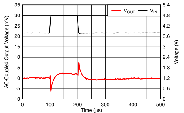
Figure 6-38. Line Transient
