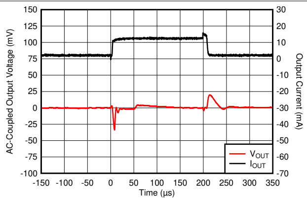
Figure 6-12. I_{OUT} Transient From 1 mA to 10 mA
