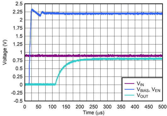
Figure 6-15. Start-Up With V_{IN} Before V_{BIAS} and V_{EN}
