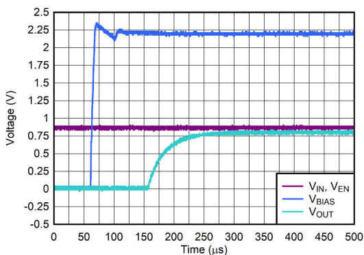
Figure 6-17. Start-Up With V_{IN} and V_{EN} Before V_{BIAS}
