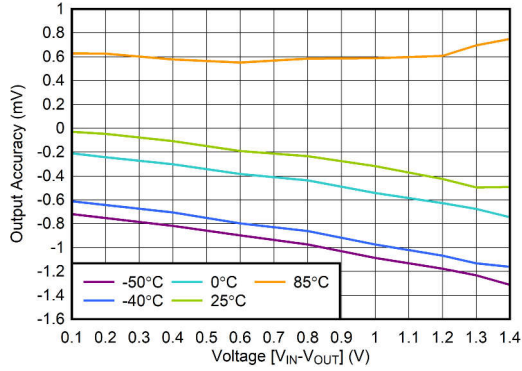
Figure 6-1. Output Voltage Accuracy vs V_{\text{IN}}
