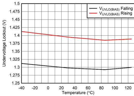
Figure 6-13. V_{BIAS} UVLO vs Temperature
