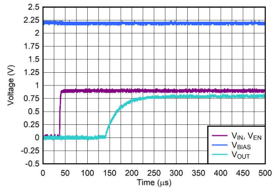
Figure 6-14. Start-Up With V_{BIAS} Before V_{IN}
