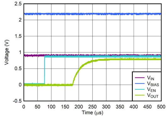
Figure 6-16. Start-Up With V_{IN} and V_{BIAS} Before V_{EN}
