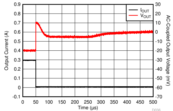
Figure 5-56. Load Transient
