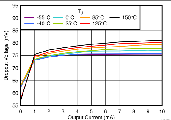
Figure 5-28. Dropout Voltage vs I_{OUT}
