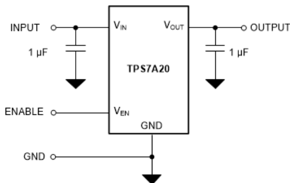
Application Schematic
