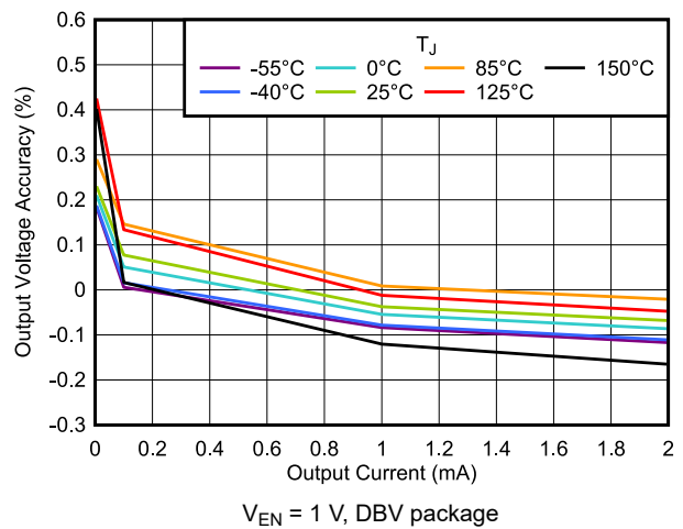
Figure 5-16. Output Voltage Accuracy vs I_{OUT}
