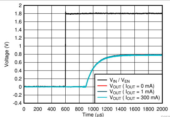
Figure 5-74. Start-Up
