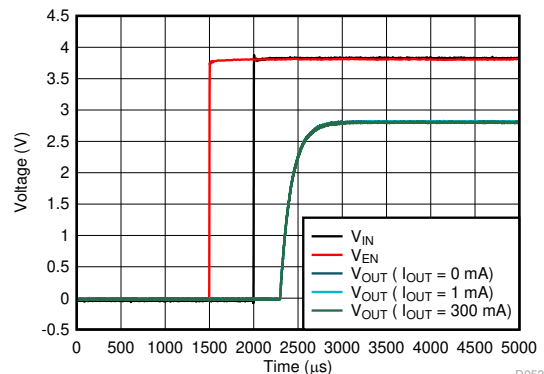
Figure 5-76. Start-Up
