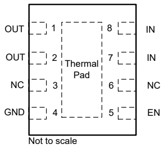
Figure 4-2. DSG Package (DSG0008B, Advance Information), 8-Pin Fixed WSON (Top View)
