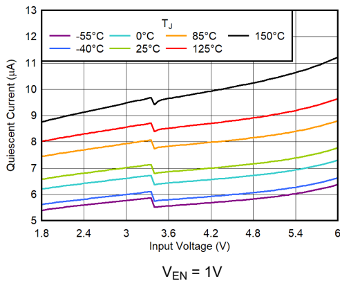
Figure 5-9. I_Q vs V_{IN}
