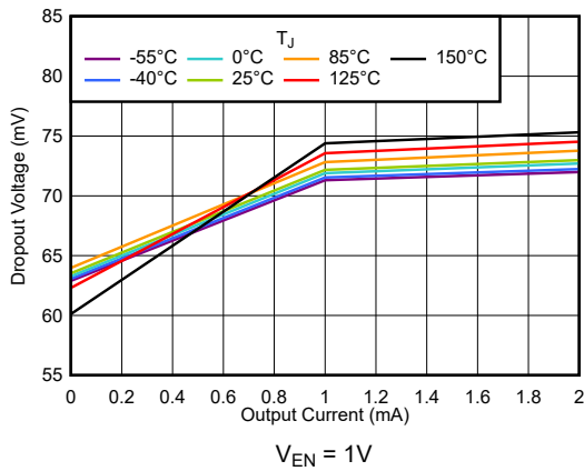
Figure 5-7. Dropout Voltage vs I_{OUT}
