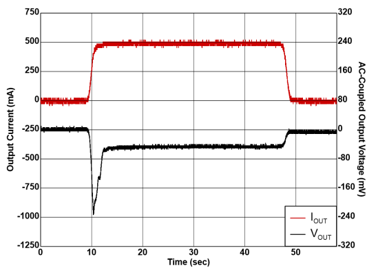
Figure 5-31. Load Transient From 0mA to 500mA
