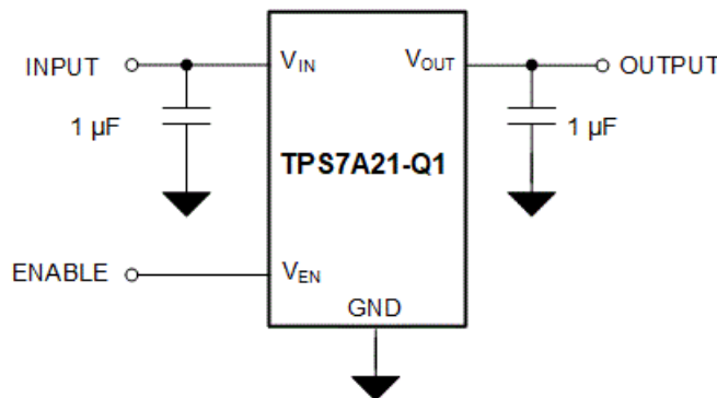
Figure 7-4. TPS7A21-Q1 Typical Application
