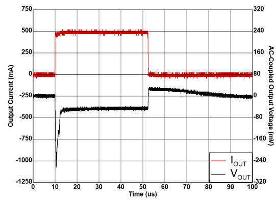
Figure 5-32. Load Transient From 0mA to 500mA
