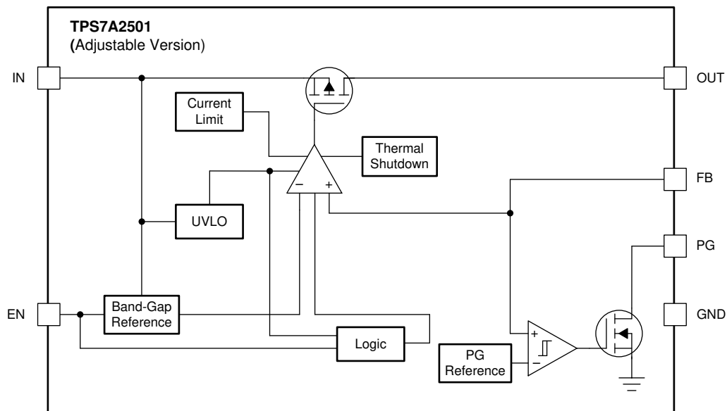
Figure 8-1. Adjustable Version
