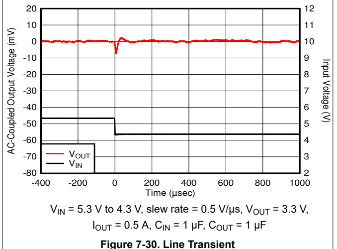
Figure 7-30. Line Transient
