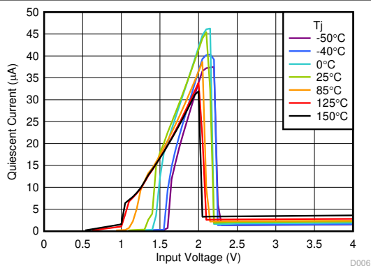
Figure 7-9. I_{GND} vs V_{IN}
