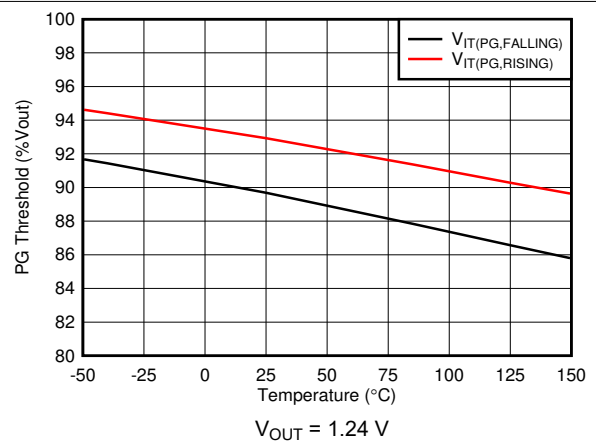
Figure 7-16. PG Thresholds vs Temperature
