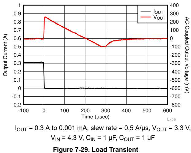
Figure 7-29. Load Transient
