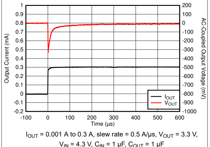
Figure 7-28. Load Transient
