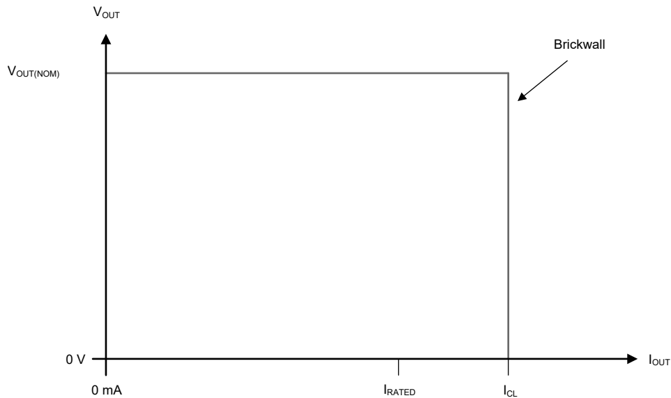
Figure 8-3. Current Limit
