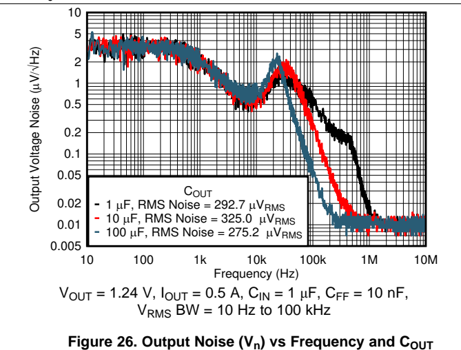
Figure 26. Output Noise ( V_n ) vs Frequency and C_{OUT}
