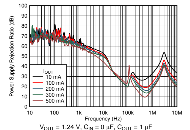
Figure 18. PSRR vs Frequency and I_{OUT}
