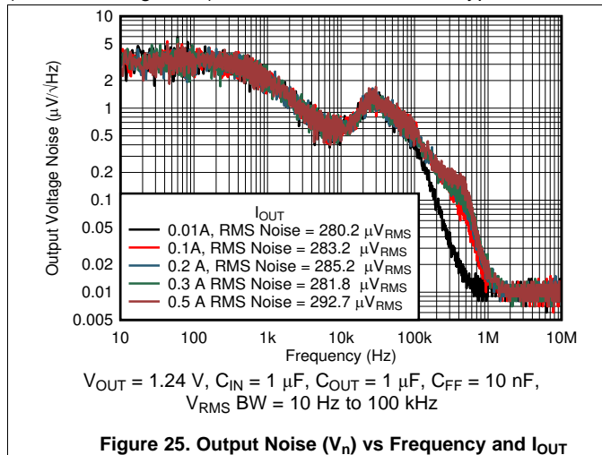
Figure 25. Output Noise ( V_n ) vs Frequency and I_{OUT}
