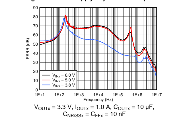
Figure 6. Power-Supply Rejection vs Input Voltage
