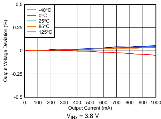
Figure 27. Load Regulation ( V_{\text{OUTX}} = 3.3\text{ V} )
