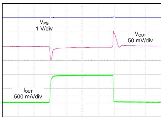
Figure 29. Load Transient Response ( V_{OUT} = 1.2\text{ V} ) V_{IN} = 1.5\text{ V} , I_{OUT} = 100\text{ mA} to 1\text{ A} to 100\text{ mA} at 1\text{ A}/\mu\text{s} , C_{OUT} = 10\ \mu\text{F} , V_{PG} = V_{OUT}
