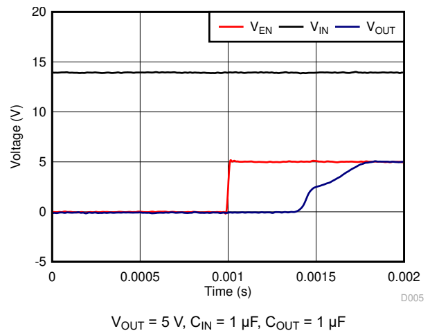
Figure 6-18. Startup With Enable
