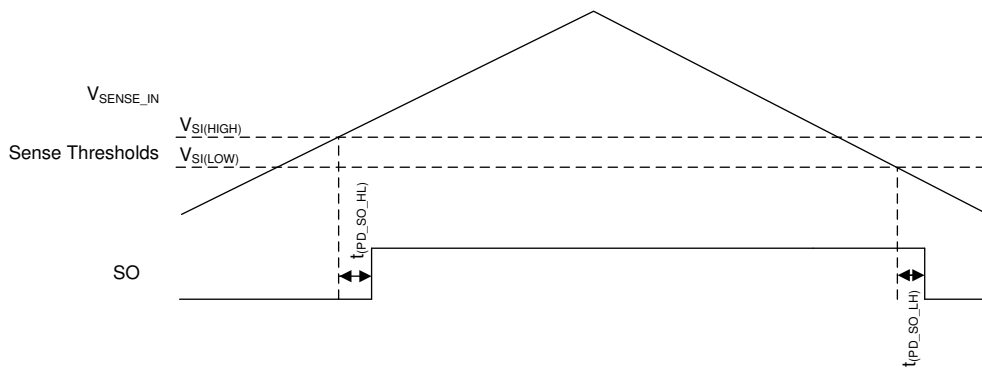
Figure 8-4. SI Timing Diagram
