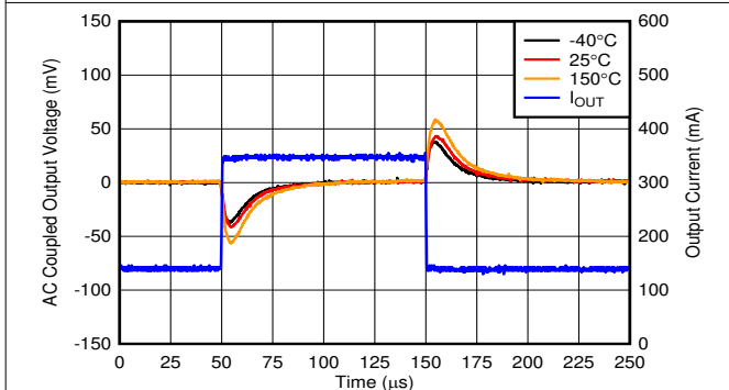
V_{OUT} = 5\text{ V} , I_{OUT} = 150\text{ mA} to 350\text{ mA} , slew rate = 0.1\text{ A}/\mu\text{s} , V_{EN} = 3.3\text{ V} , C_{OUT} = 10\ \mu\text{F}
