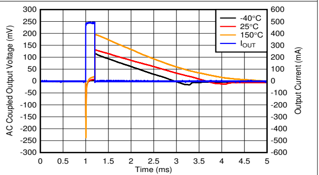
V_{OUT} = 5\text{ V} , I_{OUT} = 0\text{ mA} to 500\text{ mA} , slew rate = 1\text{ A}/\mu\text{s} , V_{EN} = 3.3\text{ V} , C_{OUT} = 10\ \mu\text{F}
