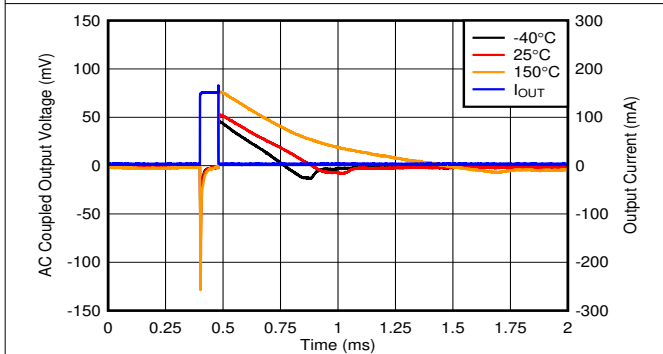
V_{OUT} = 5\text{ V} , I_{OUT} = 0\text{ mA} to 150\text{ mA} , slew rate = 1\text{ A}/\mu\text{s} , V_{EN} = 3.3\text{ V} , C_{OUT} = 10\ \mu\text{F}
