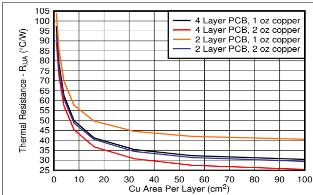
Figure 8-2. R_{\theta JA} vs Copper Area (DDA Package)
