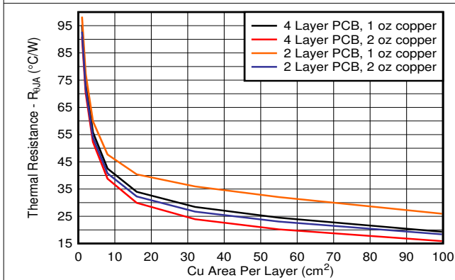
Figure 8-4. R_{\theta JA} vs Copper Area (KVU Package)
