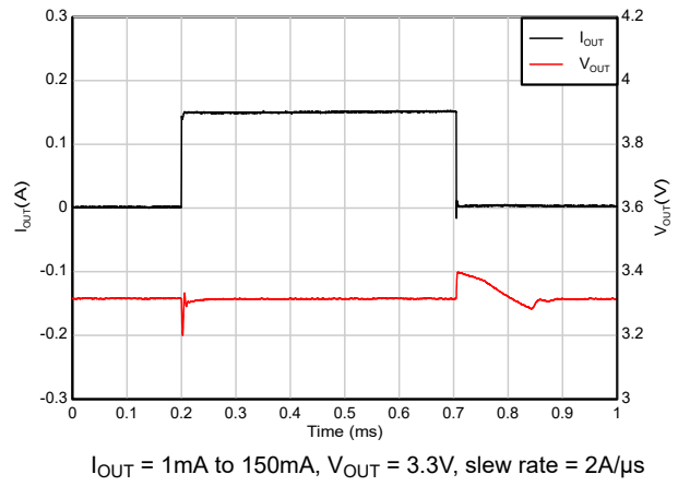
Figure 7-7. Load Transient
