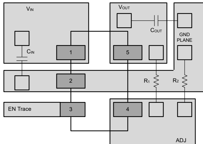
Figure 7-11. Example Layout for TPS7E71, DBV Package
