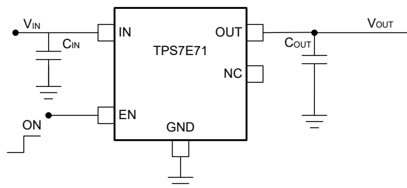
Figure 7-4. TPS7E71 Typical Application Circuit (Fixed-Voltage Version)
