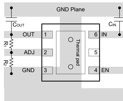
Figure 7-12. Example Layout for TPS7E71, DRV Package
