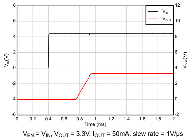
Figure 7-10. Start-up with IN and EN Tied Together
