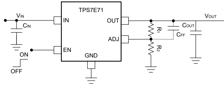
Figure 7-5. TPS7E71 Adjustable LDO Regulator Programming
