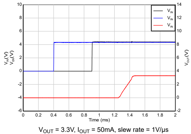
Figure 7-9. Start-up with Sequencing (IN after EN)
