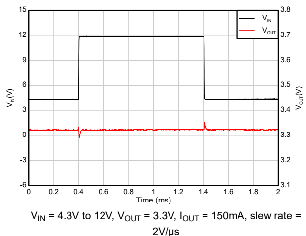
Figure 5-30. Line Transient
