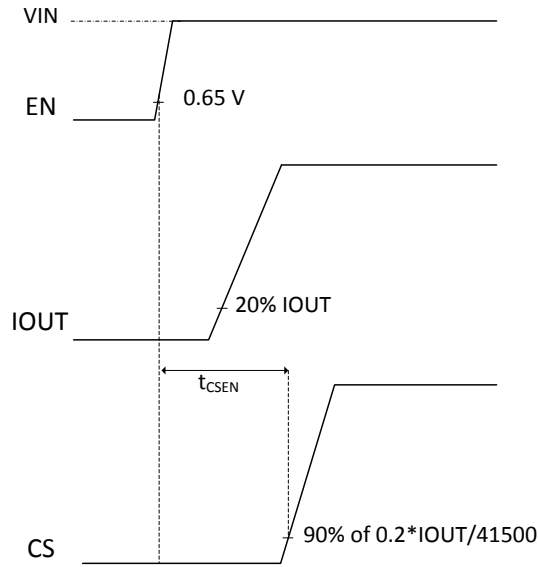
Figure 7-4. t_{CSEN} Waveforms
