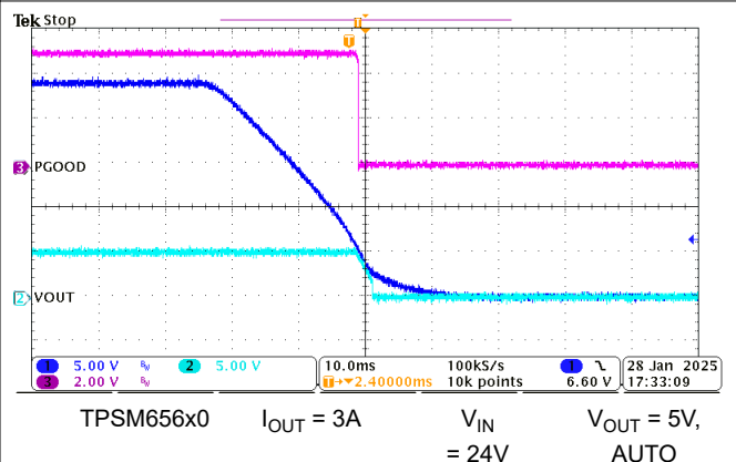
Figure 8-10. Shutdown
