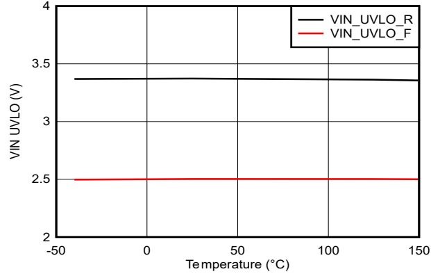
Figure 6-7. V_{IN} UVLO
