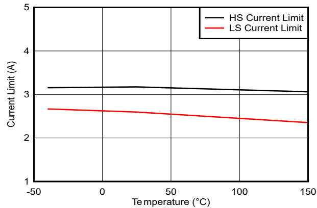
Figure 6-9. 2A Current Limit
