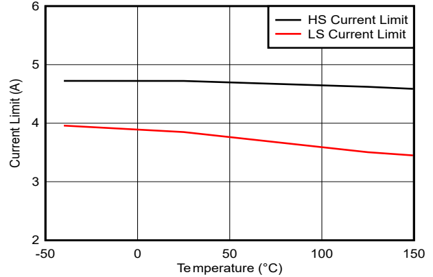
Figure 6-8. 3A Current Limit
