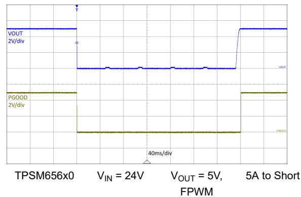
Figure 8-13. Short Circuit Applied
