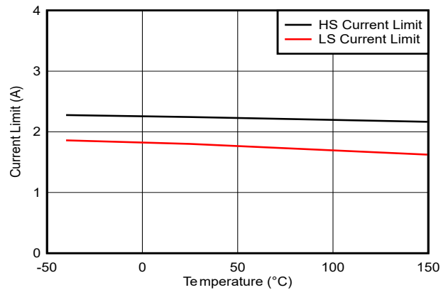
Figure 6-10. 1A Current Limit
