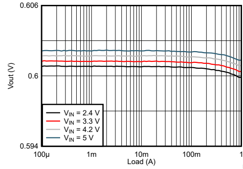
Figure 9-42. Load Regulation
