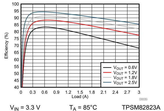
Figure 9-142. Efficiency
