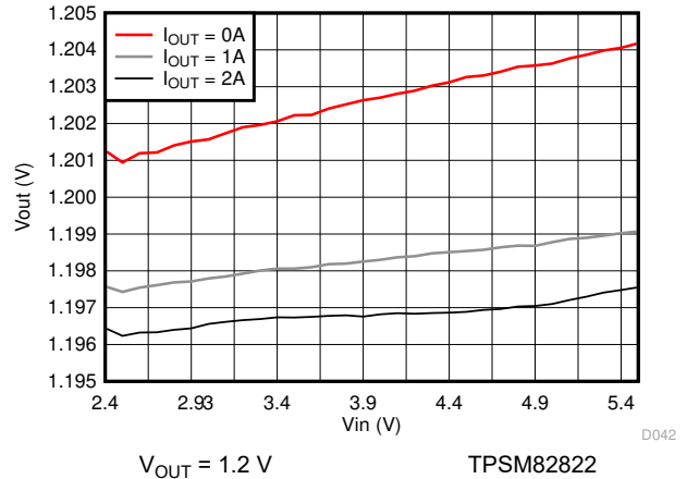
Figure 9-72. Line Regulation
