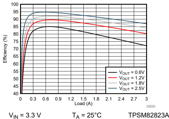
Figure 9-141. Efficiency
