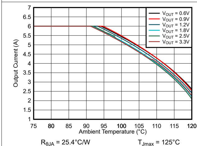
R_{\theta JA} = 25.4^\circ\text{C/W} T_{Jmax} = 125^\circ\text{C} Figure 9-30. Safe Operating Area V_{IN} = 5.0\text{ V} TPSM82866AA0HRDMR
