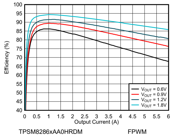
Figure 9-13. Efficiency V_{IN} = 2.8\text{ V} and T_A = 85^\circ\text{C}
