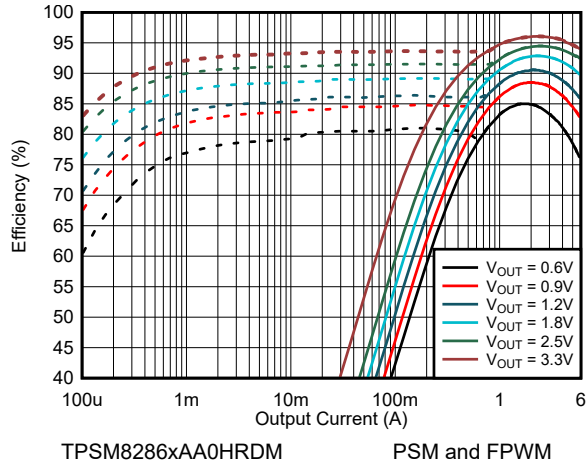
Figure 9-8. Efficiency V_{IN} = 5.0\text{ V} and T_A = 25^\circ\text{C}
