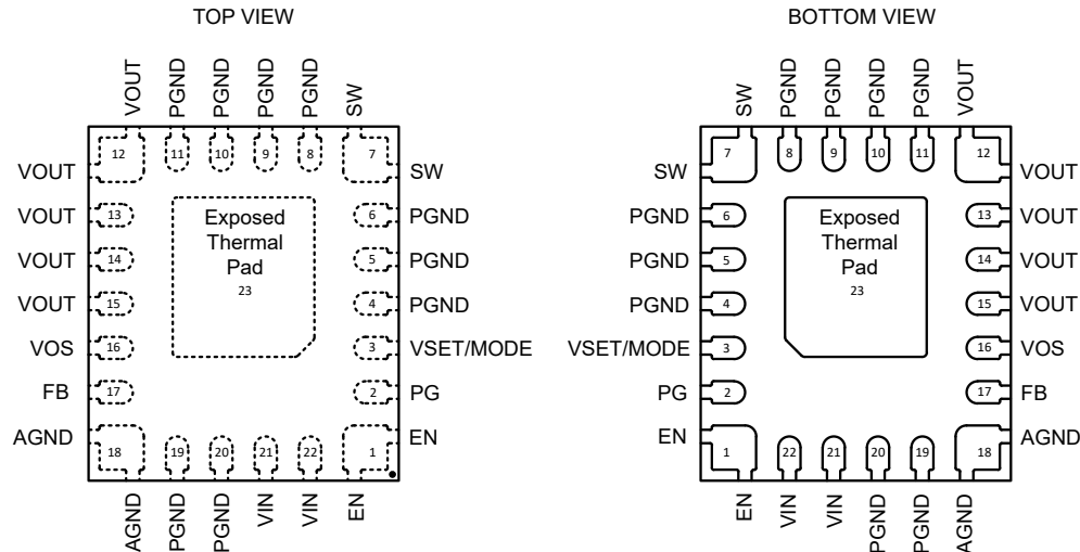
Figure 6-1. TPSM82864A, TPSM82866A - QFN (23 Pin)
