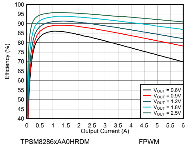
Figure 9-11. Efficiency V_{IN} = 3.3\text{ V} and T_A = 85^\circ\text{C}
