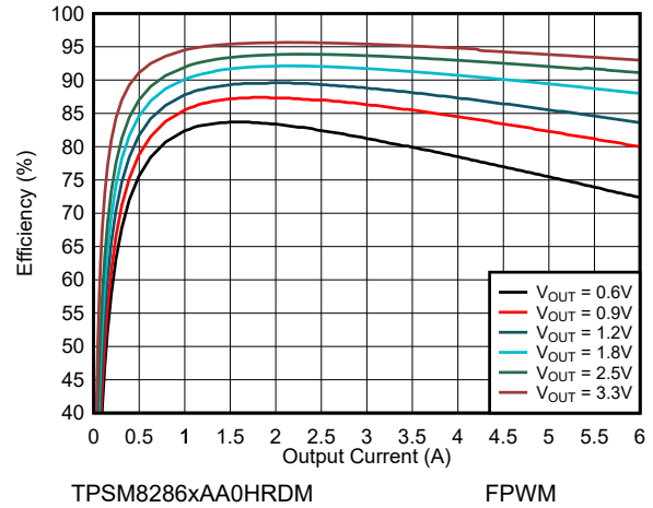
Figure 9-9. Efficiency V_{IN} = 5.0\text{ V} and T_A = 85^\circ\text{C}
