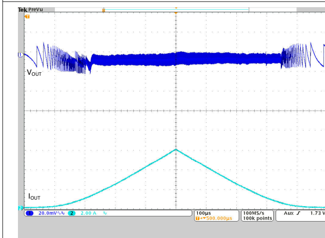
V_{IN} = 5.0\text{ V} V_{OUT} = 1.2\text{ V} T_A = 25^\circ\text{C} Figure 9-28. Load Sweep I_{OUT} = 20\text{ mA} \rightarrow 6\text{ A}
