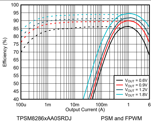
Figure 9-6. Efficiency V_{IN} = 2.8\text{ V} and T_A = 25^\circ\text{C}
