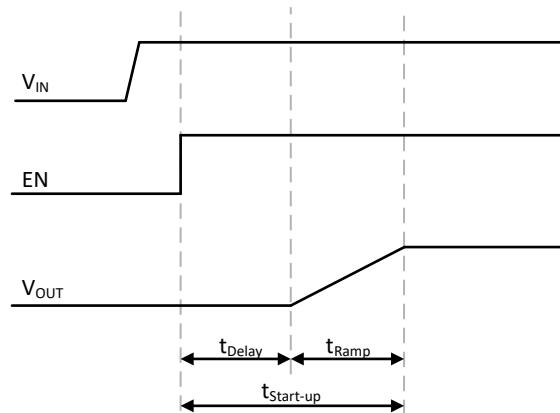
Figure 8-2. Start-Up Sequence
