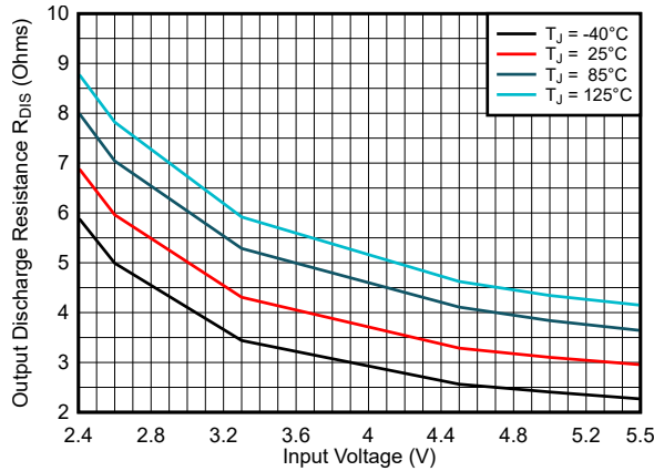
Figure 7-3. Output Discharge Resistance R DIS
