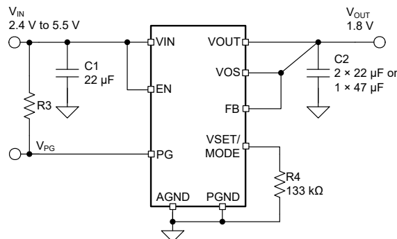
Figure 8-4. Fixed Output Voltage Application Circuit
