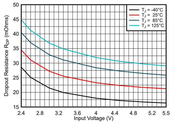
Figure 7-5. Dropout Resistance R DP
