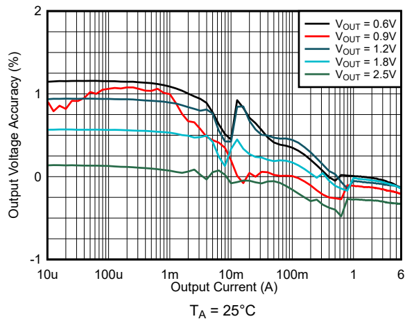
Figure 9-16. Load Regulation V_{IN} = 3.3\text{ V} and PSM
