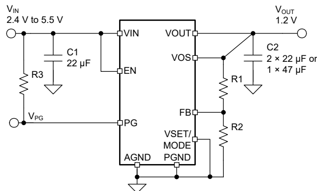
Figure 9-1. Typical Application
