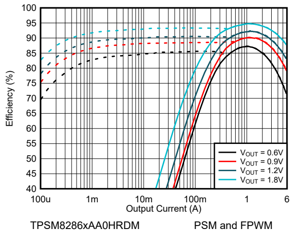
Figure 9-12. Efficiency V_{IN} = 2.8\text{ V} and T_A = 25^\circ\text{C}
