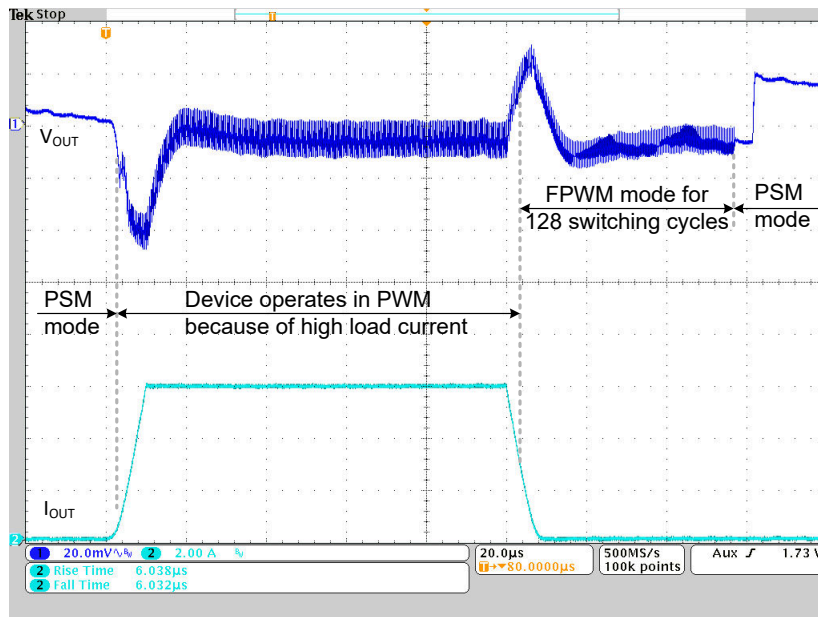
Figure 8-1. Optimized Transient Performance from PWM to PSM
