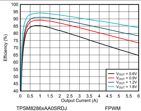
Figure 9-7. Efficiency V_{IN} = 2.8\text{ V} and T_A = 85^\circ\text{C}
