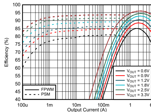
TPSM82866AA0HRDMR – Efficiency Versus Output Current; V_{IN} = 5.0\text{ V}
