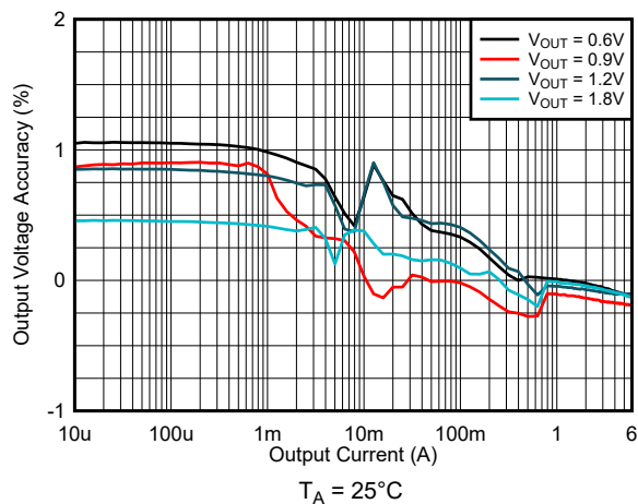
Figure 9-18. Load Regulation V_{IN} = 2.8\text{ V} and PSM
