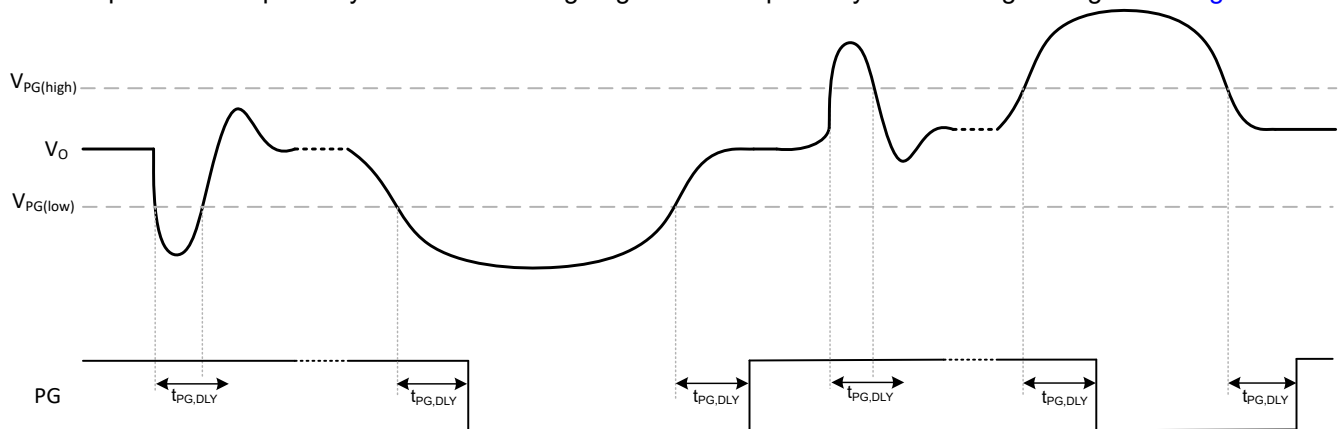
Figure 8-3. Power-Good Transient and Delay Behavior
