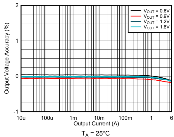
Figure 9-19. Load Regulation V_{IN} = 2.8\text{ V} and FPWM
