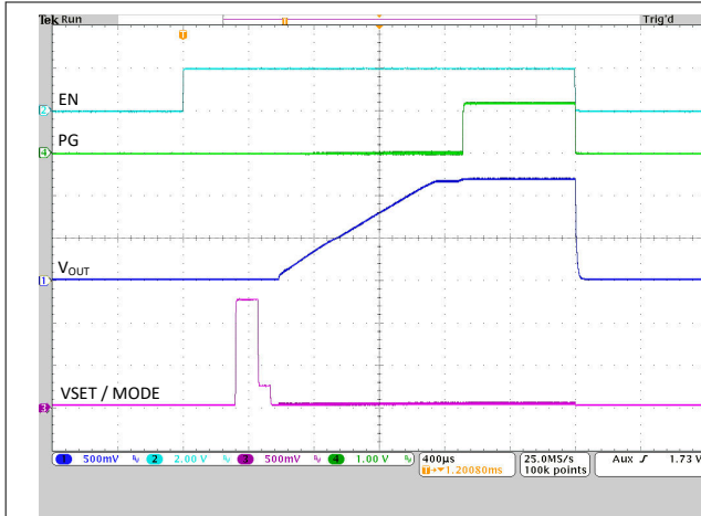
R_{VSET} = 56.2\text{ k}\Omega I_{OUT} = 6.0\text{ A} Figure 9-26. Start-Up into Full Load
