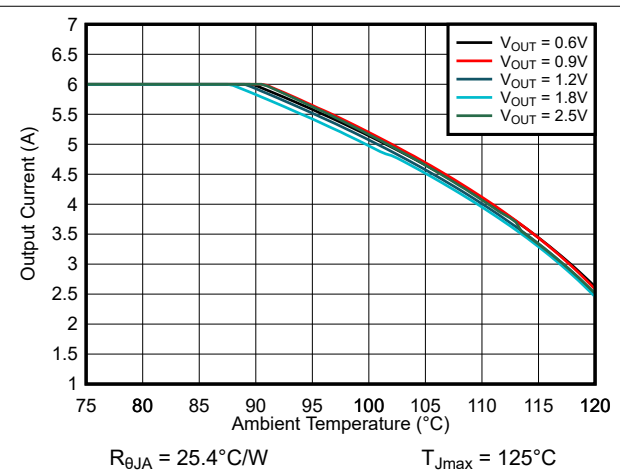
R_{\theta JA} = 25.4^\circ\text{C/W} T_{Jmax} = 125^\circ\text{C} Figure 9-31. Safe Operating Area V_{IN} = 3.3\text{ V} TPSM82866AA0HRDMR
