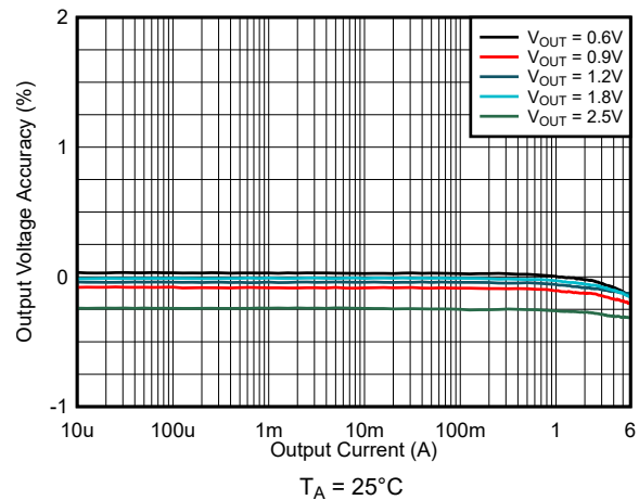
Figure 9-17. Load Regulation V_{IN} = 3.3\text{ V} and FPWM
