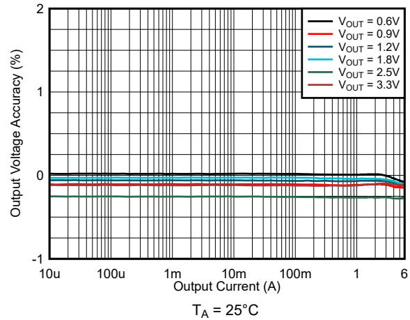
Figure 9-15. Load Regulation V_{IN} = 5.0\text{ V} and FPWM
