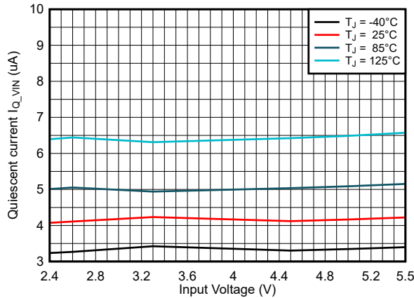
Figure 7-1. Quiescent Current into V IN I Q_VIN
