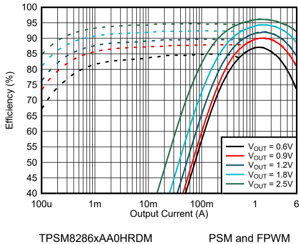
Figure 9-10. Efficiency V_{IN} = 3.3\text{ V} and T_A = 25^\circ\text{C}
