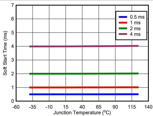
Figure 5-11. Soft Start
