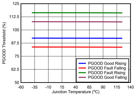
Figure 5-9. PG Threshold
